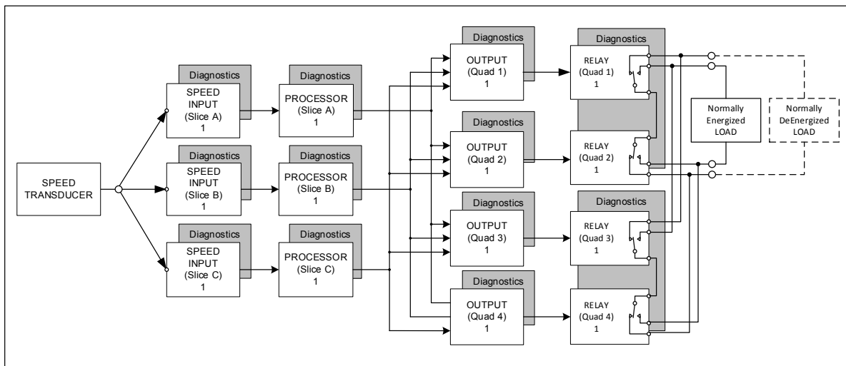
Figure 1 Module Architecture
